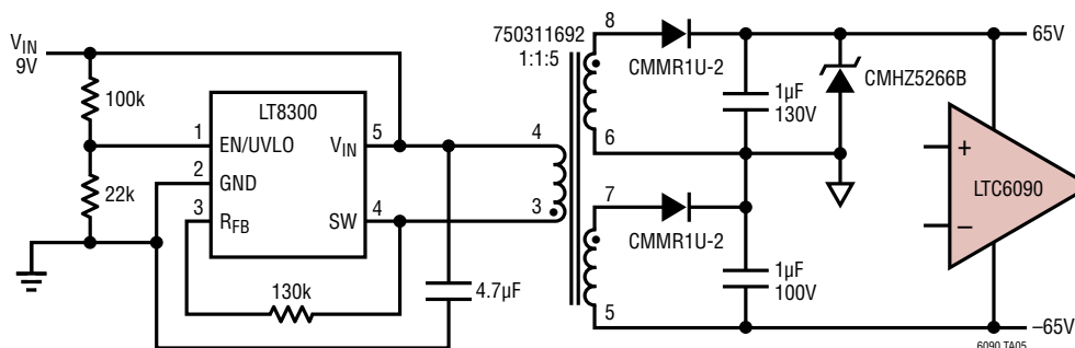
9V to ±65V Isolated Flyback Converter for Amplifier Supply
